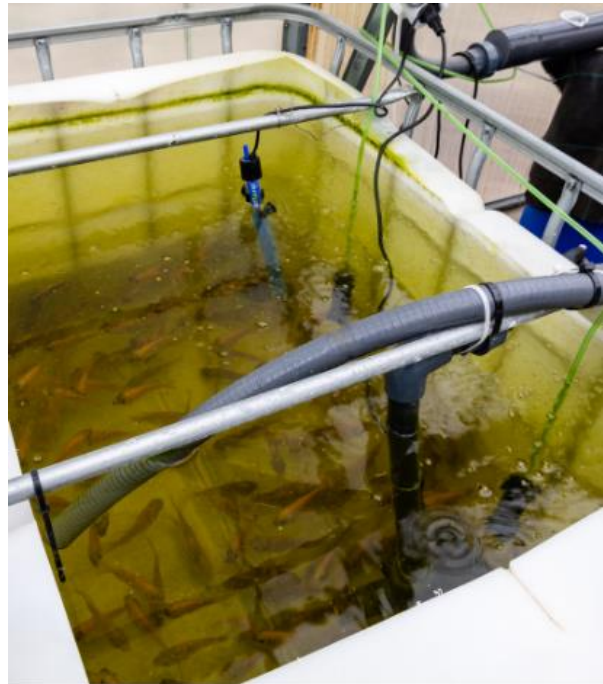
Figure 11. An IBC (Euro-cube) used for fish cultivation in an aquaponics system.
