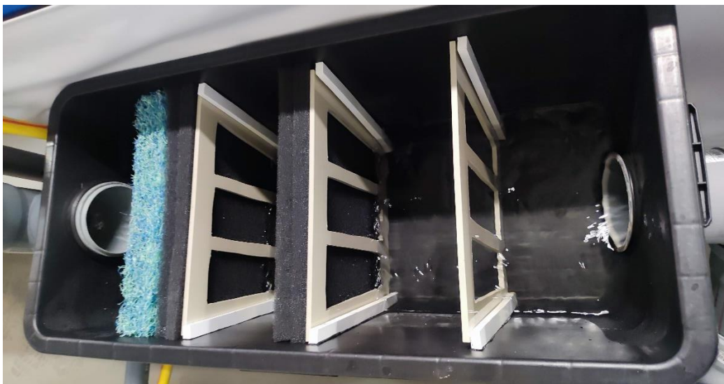
Figure 12. A mechanical filter for sludge removal in an aquaponics system.
