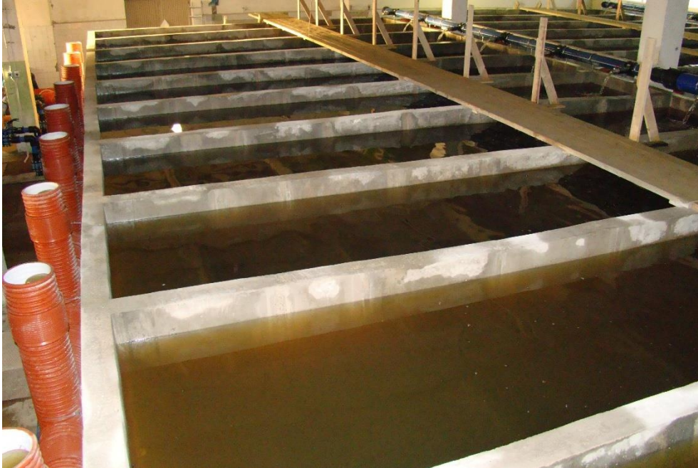
Figure 10. Concrete fish tanks in Latvian aquaculture system. 2
