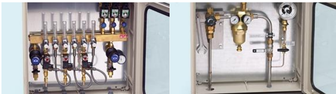
Figure 2. Linde Gas O 2 flow or dosing box and emergency O 2 box.
